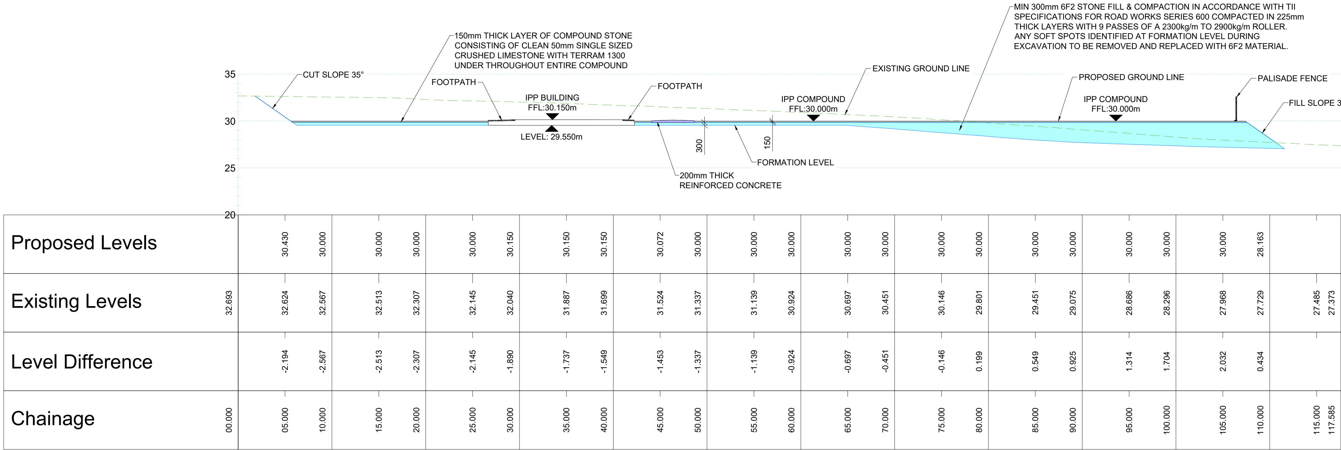
SECTION D-D CH0.0M TO 117.6M SCALE H 1:250 , V 1:250
