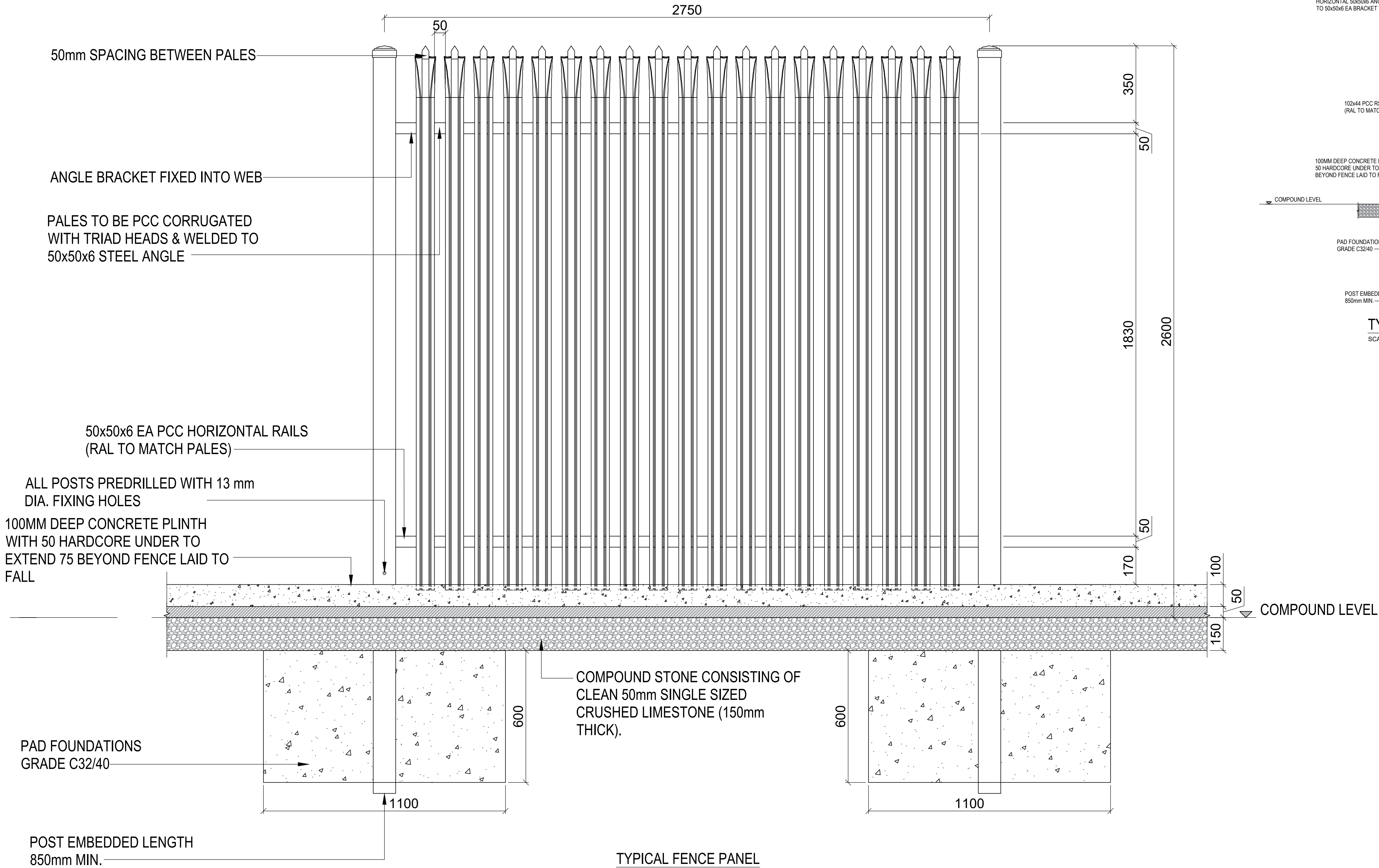
TYPICAL FENCE PANEL ELEVATION SCALE 1: 10
