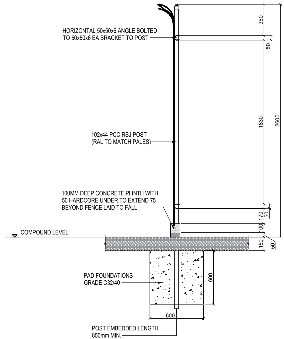
TYPICAL DETAIL SECTION SCALE 1: 25
